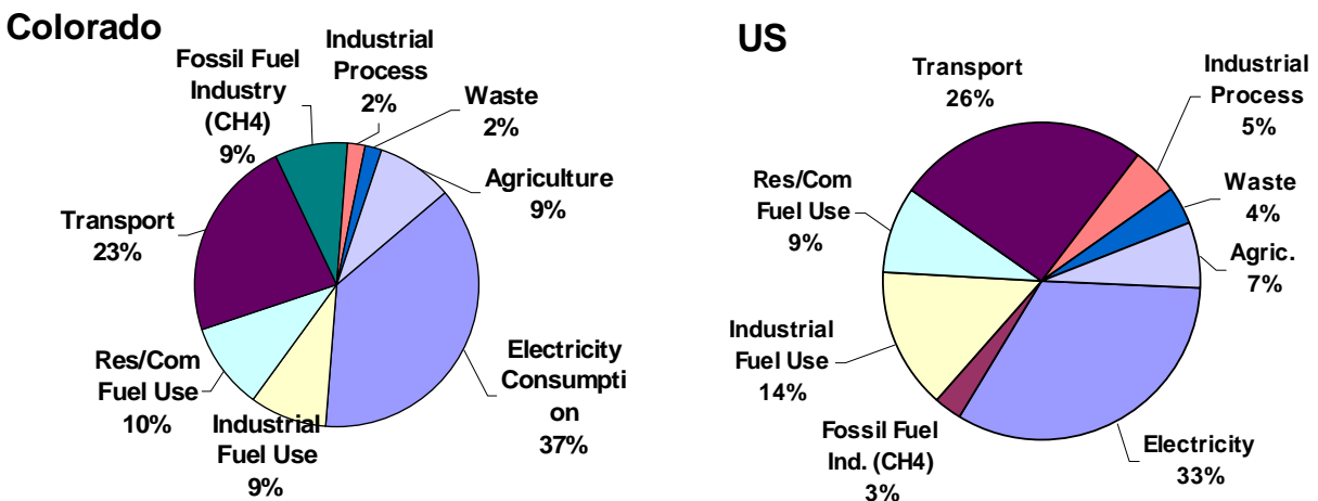
Figure 2. Gross GHG Emissions by Sector, 2000, Colorado and US
