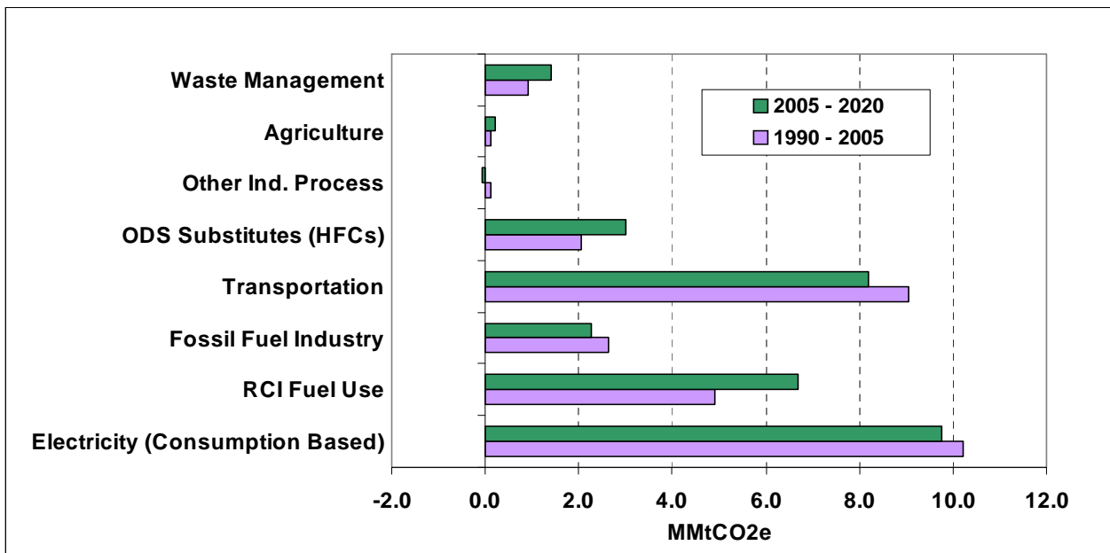
Figure 4. Sector Contributions to Gross Emissions Growth in Colorado, 1990-2020: Historic and Reference Case Projections (MMtCO 2 e Basis)
