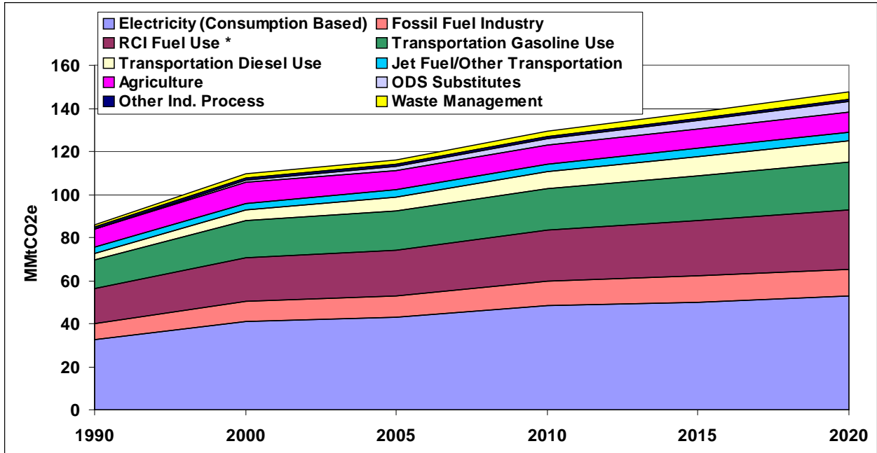
Figure 3. Colorado Gross GHG Emissions by Sector, 1990-2020: Historical and Projected
