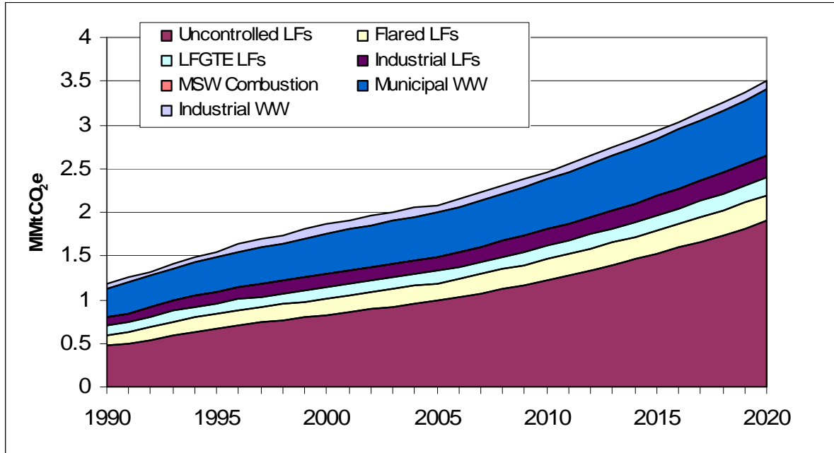
Figure G1. Colorado GHG Emissions from Waste Management
