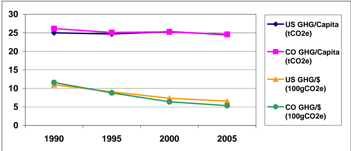
Figure ES-1. Historical Colorado and US Gross GHG Emissions, Per Capita and Per Unit Gross Product
